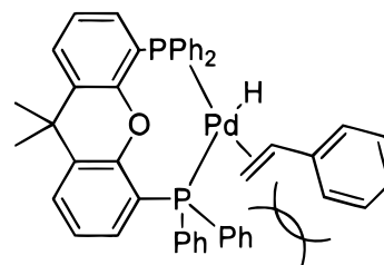
Figure 5. Increased steric hindrance of the ligands with larger bite angles between the styrene substrate and the ligand.
